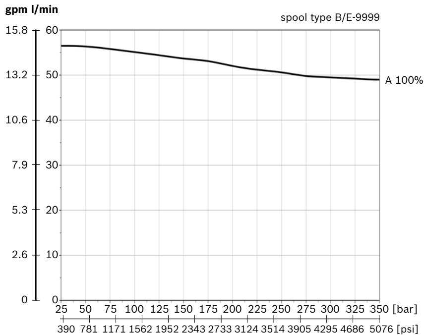
2-way inflow controller
