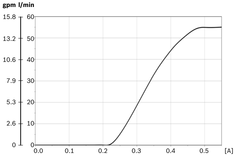
Characteristic curves Q=Q(I) at 6bar
