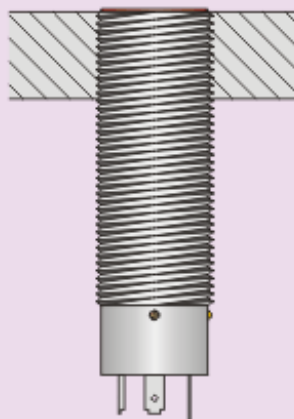
Flush mounting
