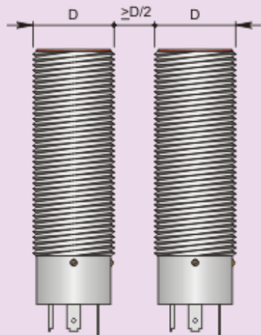
Side by side mounting
