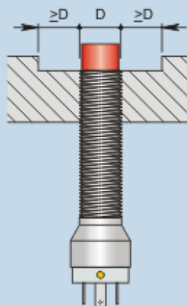
Non flush mounting
