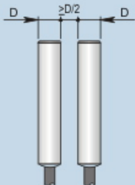
Side by side mounting
